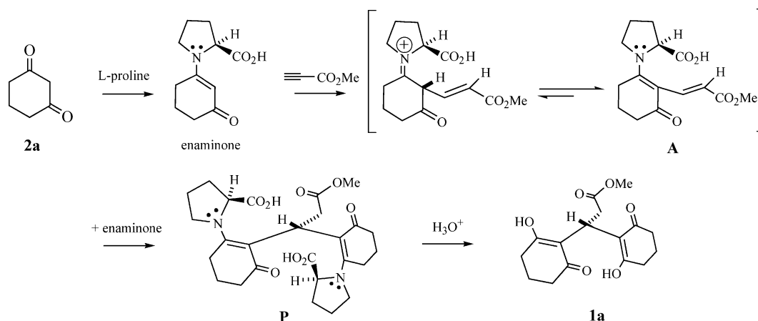
Scheme 3. Mechanism for the Michael/Michael addition of 2a .
