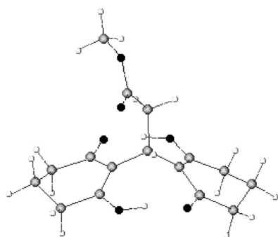
Figure 3. Top: superimposed conformational energy diagram for 1a : single point (AM1), Hartree–Fock (HF), and (density functional theory, DFT). Bottom: representation of the global minimum energy conformation of 1a .
