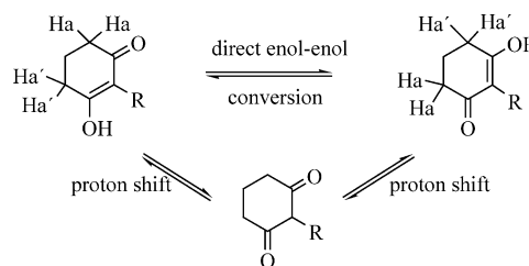
Figure 2. Tautomerization process for the dicarbonyl compounds 1 .
