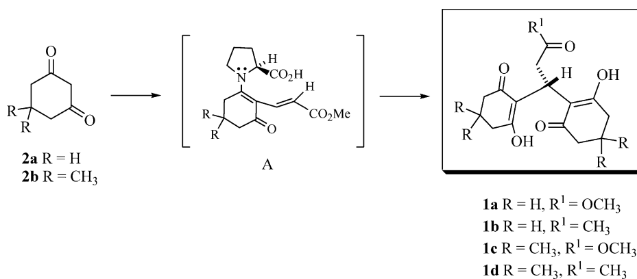
Scheme 1. Preparation of 1 by a tandem-Michael/Michael process. Reagents and conditions: \equiv\text{C(O)R}^1 (R 1 = CH 3 , OCH 3 ), DMSO, cat. L-proline, room temp.
