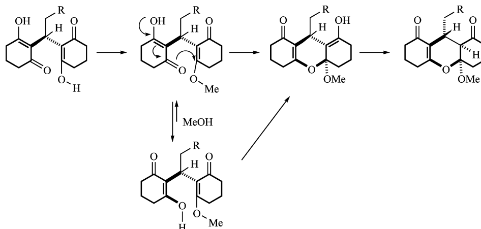
Scheme 4. Reaction mechanism for the transformation 1 → 4 with diazomethane in methanol.
