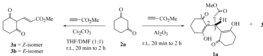
Scheme 2. Michael addition of 2a to methyl propiolate in solution and on a solid support.
