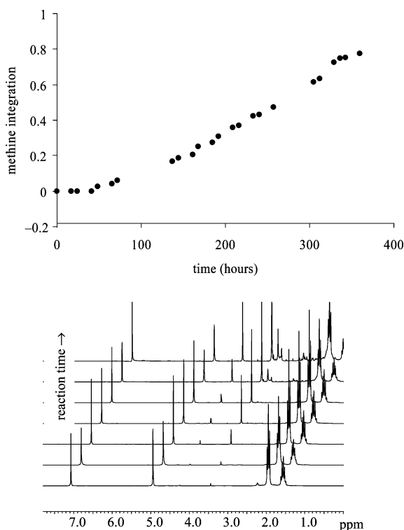
Figure 1. Top: concentration of P , as determined by methine signal integration, vs. reaction time when tandem-Michael addition of 2a was carried out by catalysis with L-proline. Bottom: ^1\text{H} NMR spectral stack plot of the reaction \mathbf{2a} \rightarrow \mathbf{P} recorded by the periodic spectral lecture ^1\text{H} NMR method. The behavior of the \text{OCH}_3 ( \delta = 3.70 ppm) and \text{CH} ( \delta = 4.50 ppm) groups of P during the reaction was considered in the calculation of the degree of conversion.
